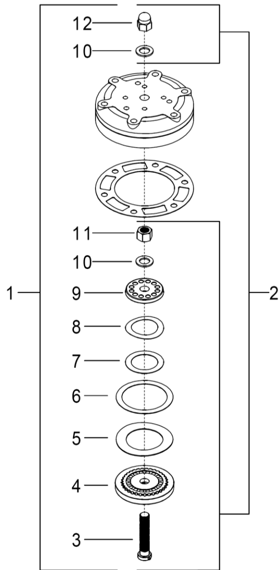
FIGURE 4 FIRST STAGE CONCENTRIC RING VALVE ASSEMBLY
