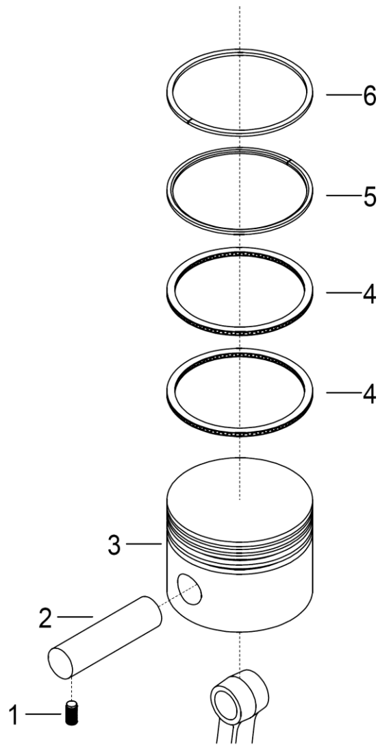
FIGURE 6 FIRST STAGE (LOW PRESSURE) CYLINDER & PISTON
