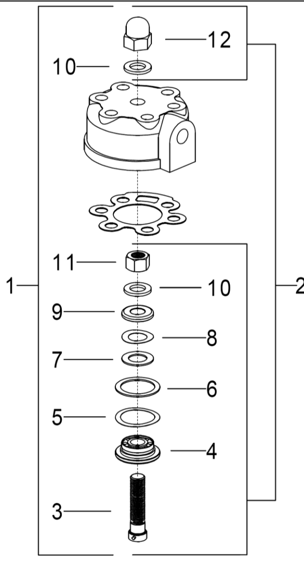
FIGURE 3 SECOND STAGE CONCENTRIC RING VALVE ASSEMBLY
